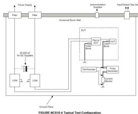
FIGURE NCS10-4 Typical Test Configuration.
