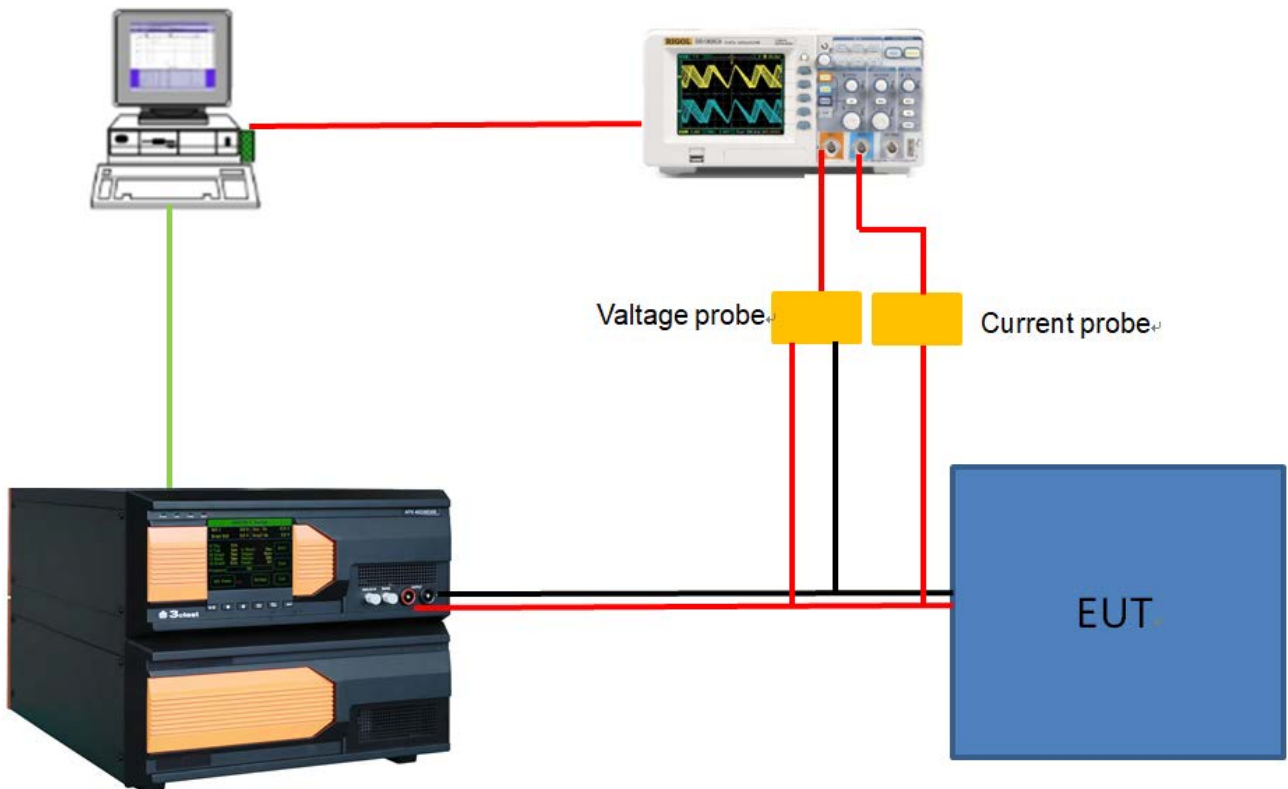
System overall connection diagram
