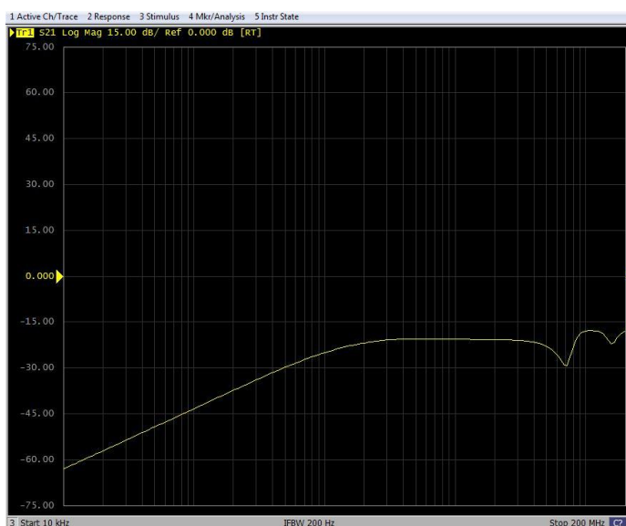
Curve S21 of TWCM-200
